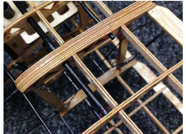
Install outer wing panels with their lineup rods.
