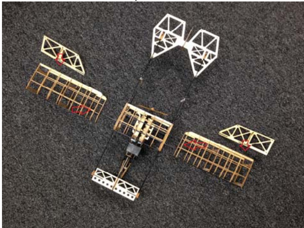
Airplane parts
