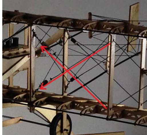
Hook up wing wires
